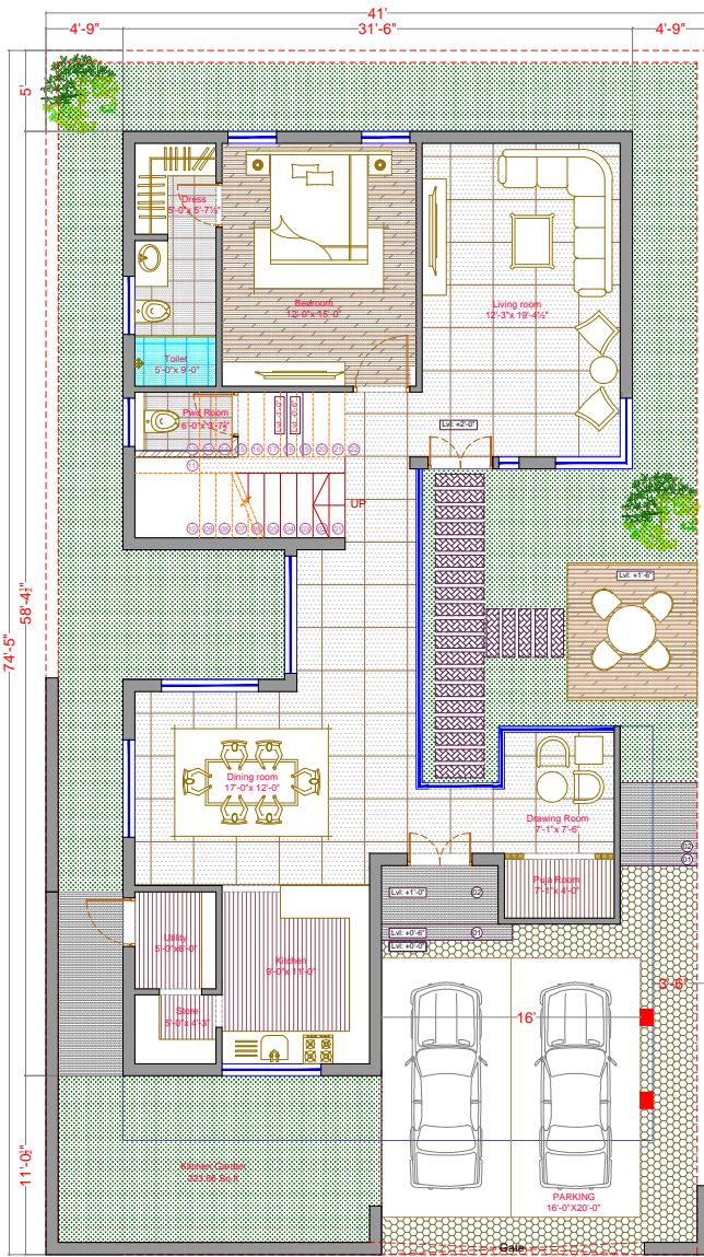
01 GROUND FLOOR PLAN 340 Sq.yds east facing villa
