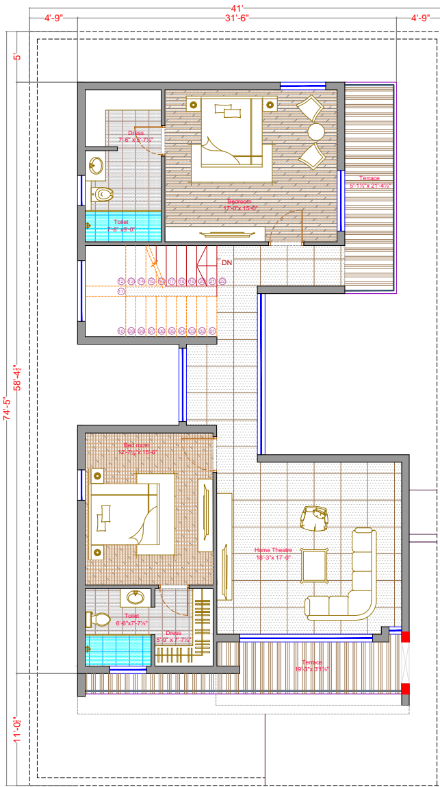
02 FIRST FLOOR PLAN 340 Sq.yds east facing villa
