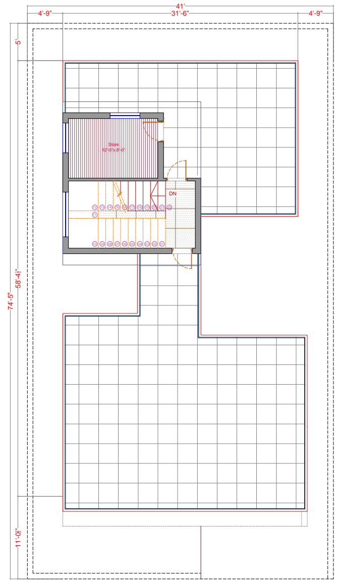
03 TERRACE FLOOR PLAN 340 Sq.yds east facing villa
